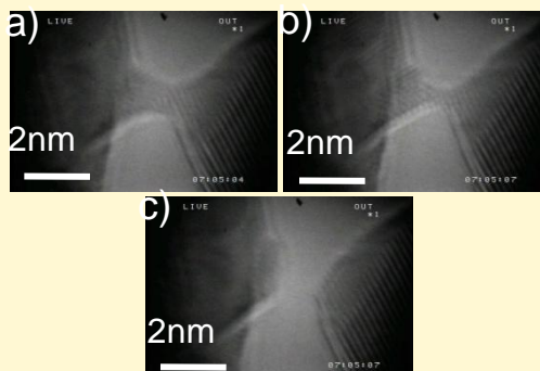
TEM images of a gold nanocontact during a tensile test
